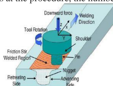
Friction stir welding schematic diagram
